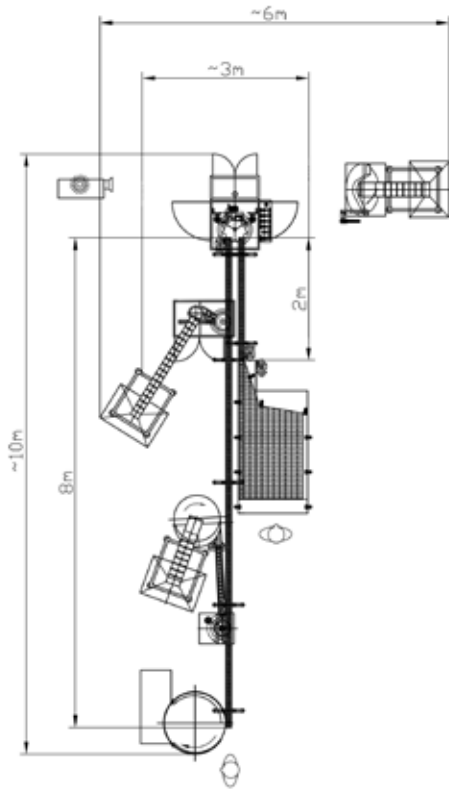
Compact Aerosol Filling Line up to 40 cans per minute
